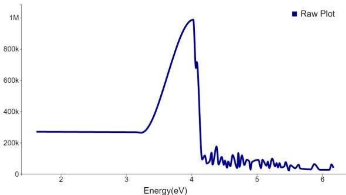
Figure 4.5 Tauc plot of optical band gap of Ag 2 ZnO thin films for sample 2
