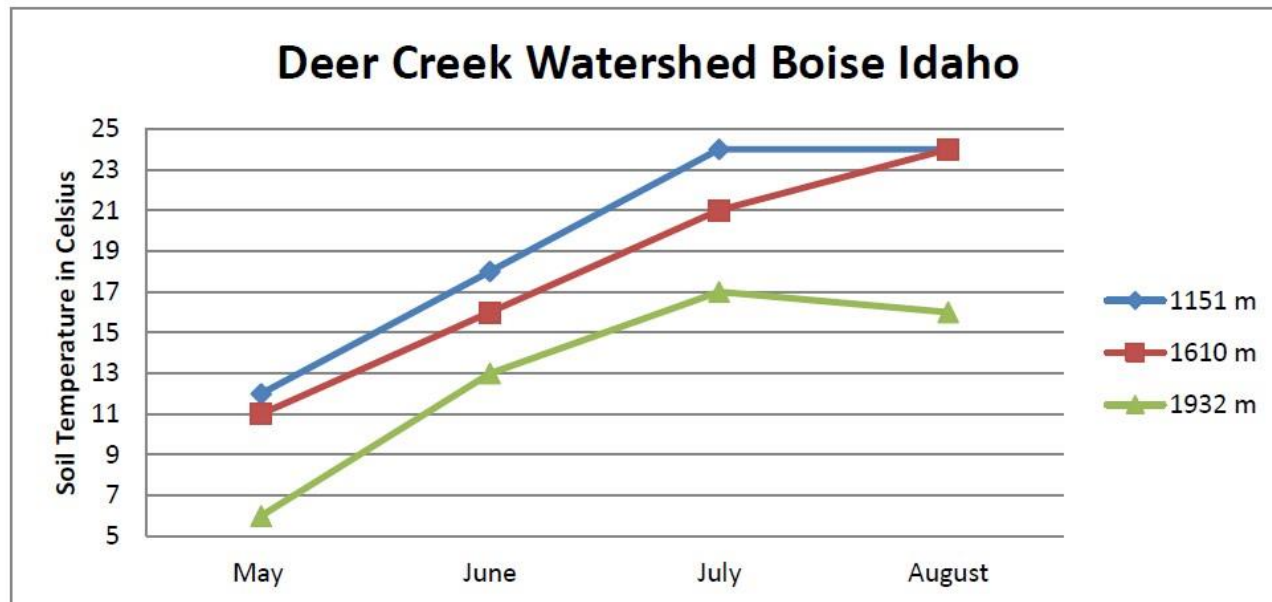
Figure 1. Deer Creek Experimental Watershed in Boise Idaho soil temperature decreases as elevation increase.
