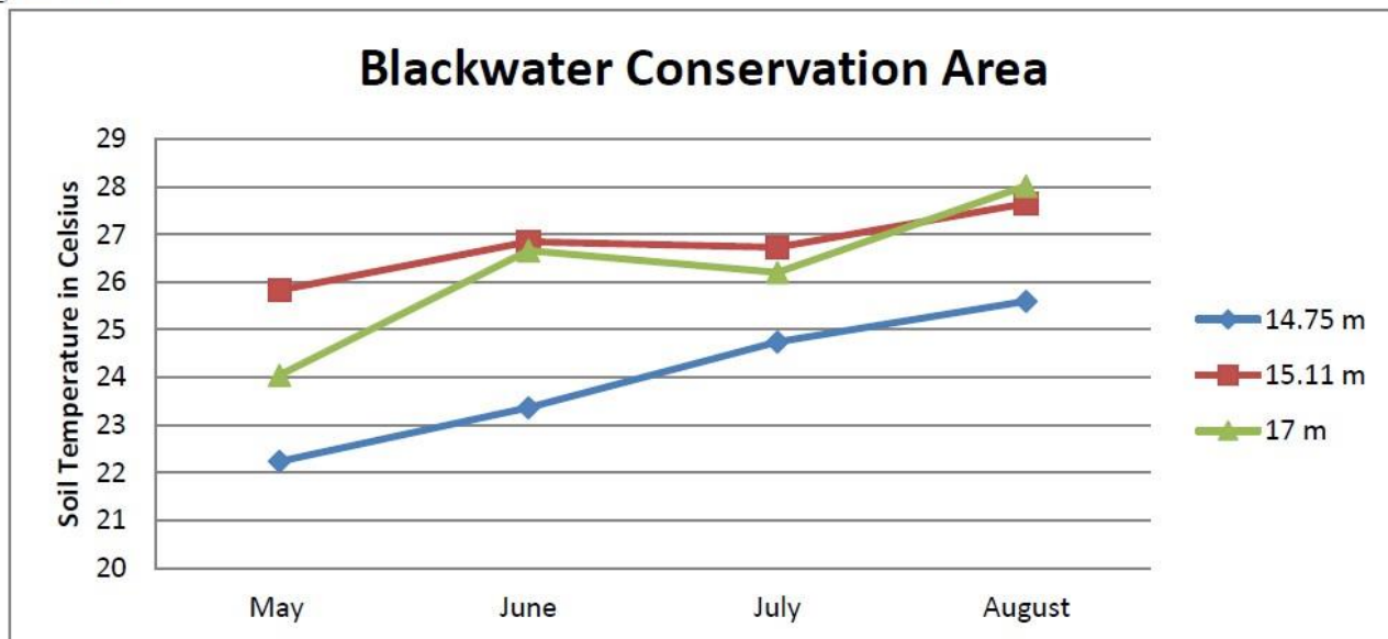
Figure 3. Soil temperature in the bottomland (14.75 m) is consistently lower than the upland (17 m) and shrub/scrub (15.11) areas. The upland and shrub/scrub areas soil temperatures alternate positions in July and August.
