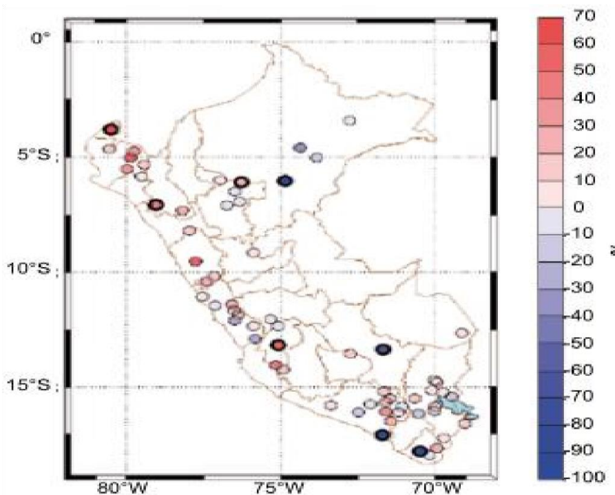
Figure 5. Linear Trend of total annual precipitation in percentage, relative to the multiannual average (1965-2006).
