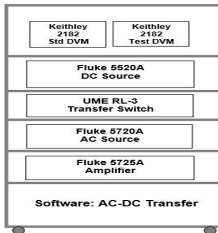
Fig. 6: Equipment Used in Calibration System
