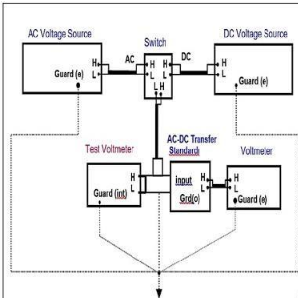
Fig. 9: Set-up of AC Function of Voltmeter
