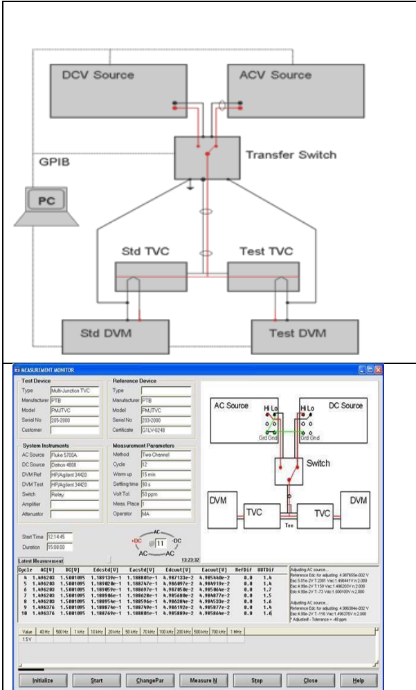
Fig. 5: A new Automated Calibration System in NMCC
