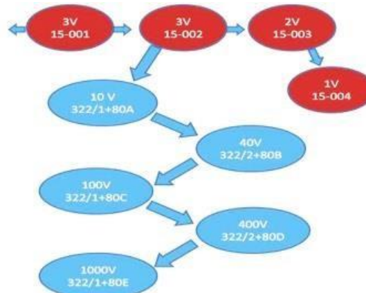
Fig. 3a: Chain of Range-to-range Build-up Measurements
