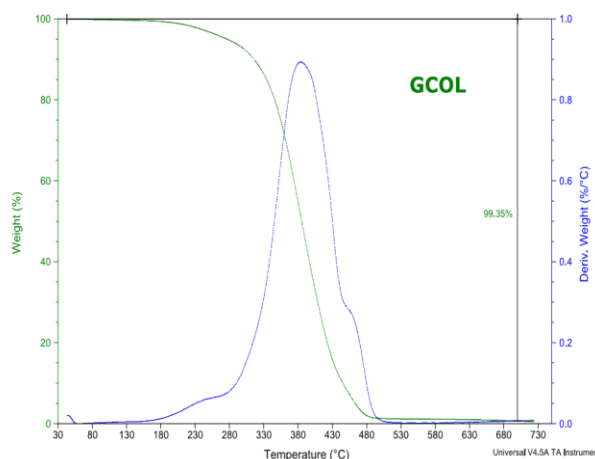
Figure 7(b) TGA plot of GCOL polyol
