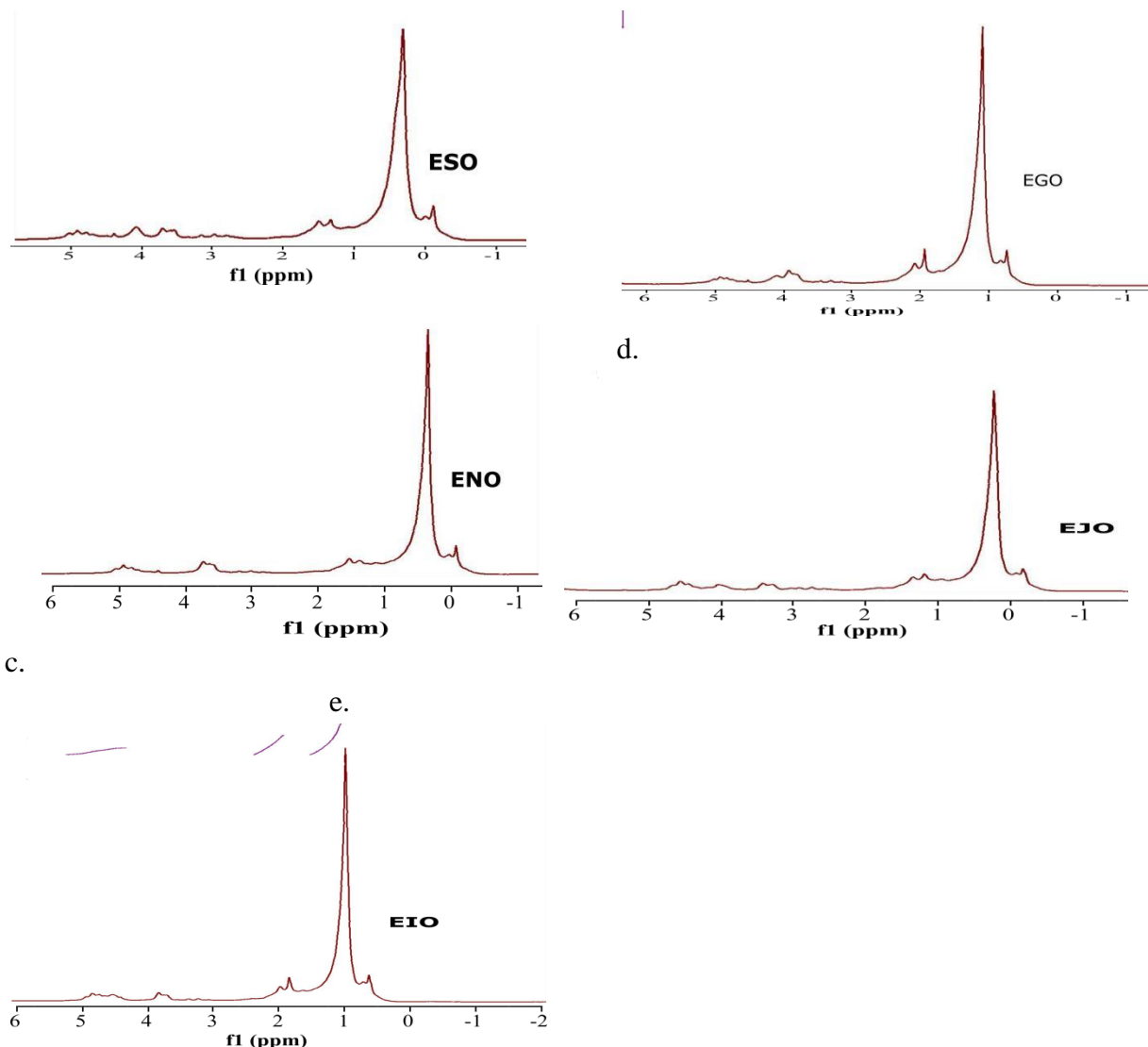
Figure. 2(a) to 2(e) ^1\text{H} NMR spectra of epoxidised vegetable oils.
