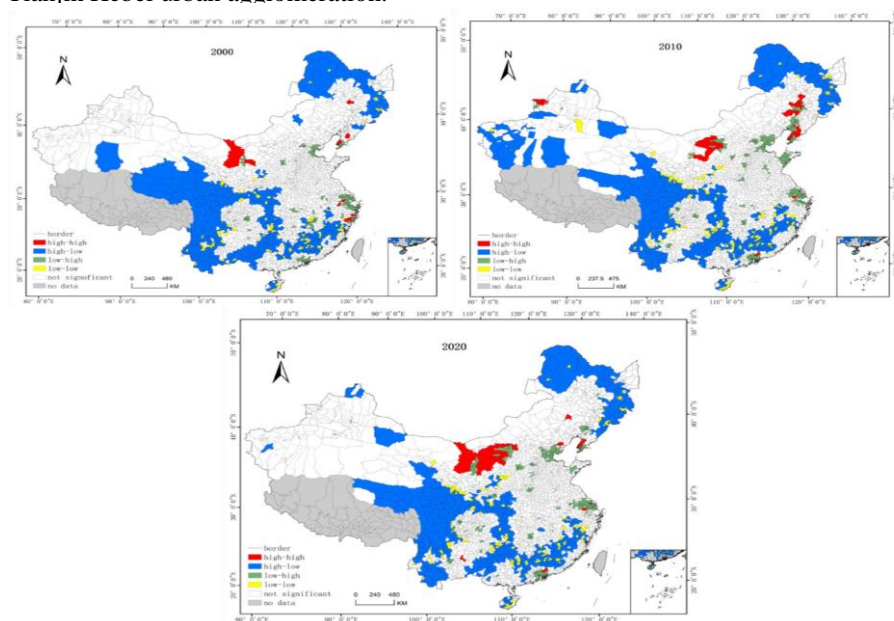
Fig. 4 LISA clustering of land use carbon emissions and ESV in Chinese counties, 2000-2020
