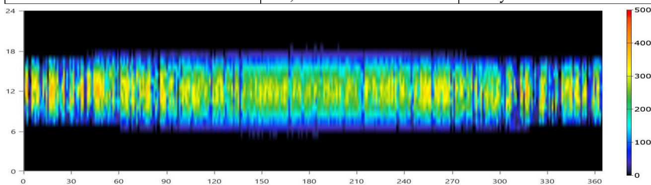
Fig. 5. Power output Huawei SUN2000 30kW with Generic PV (kW)
