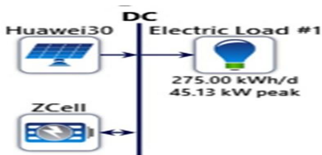
Fig. 4. Solar system in orchard
