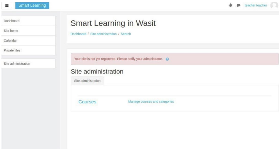
Fig. 3. Teacher's interface
