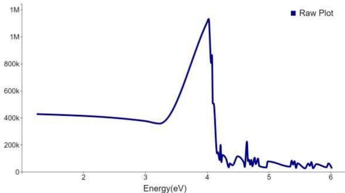
Figure 4.5 Tauc plot of optical band gap of Ag_ZnO thin films for sample 2
