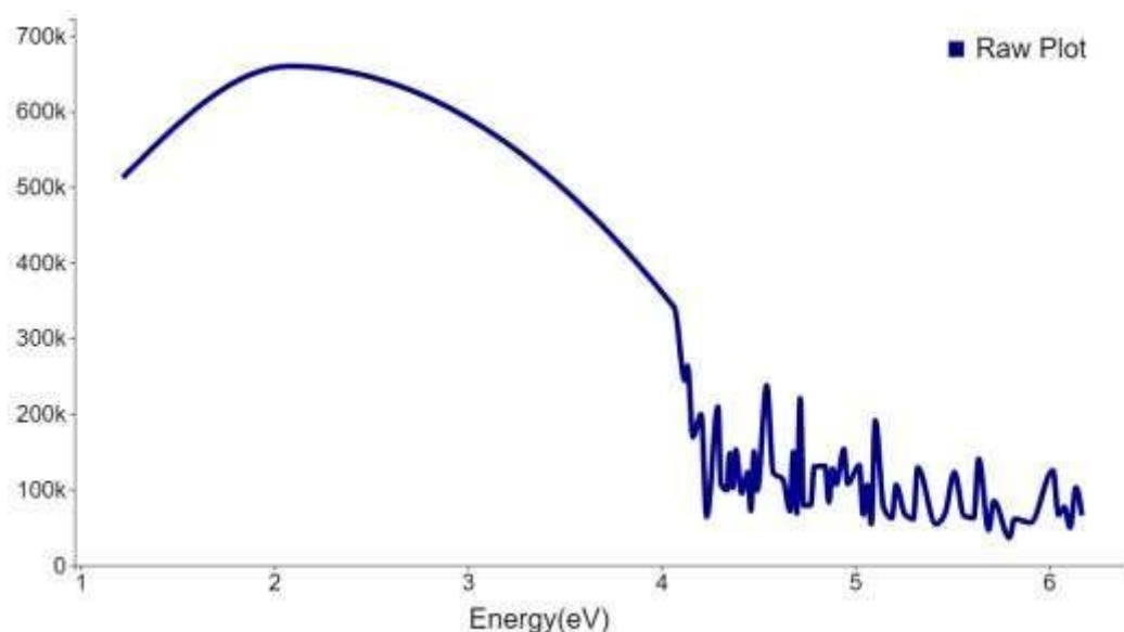
Figure 4.8 Absorbance as a function of energy band gap for sample 5
