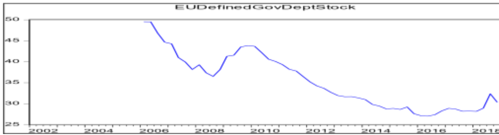
Graph 2. EUDefinedGovDeptStock
