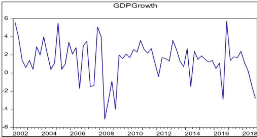
Graph 6. RIRComCredits
