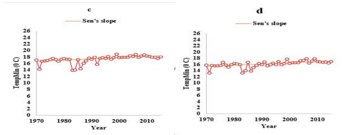
Figure 5. Fluctuation of minimum temperature over the four-crop growing seasons (a) Aus, (b) Aman, (c) Boro and (d) Wheat, Sylhet, Bangladesh (1970-2018).
