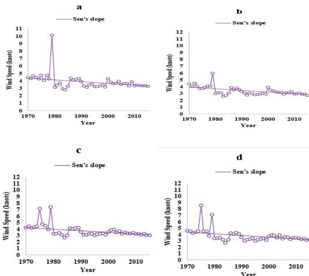
Figure 9. Variation of wind speed over the four-crop growing seasons (a) Aus, (b) Aman, (c) Boro and (d) Wheat, Sylhet, Bangladesh (1970-2018).
