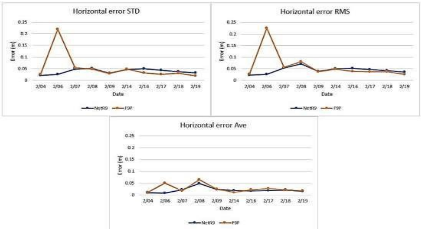
Figure 6: Horizontal error statistics plot
