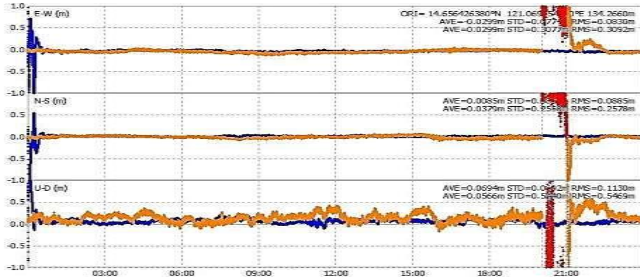
Figure 11: NetR9 (Blue) and MSJ Real-time (Orange and Red) (March 1, 2020)
