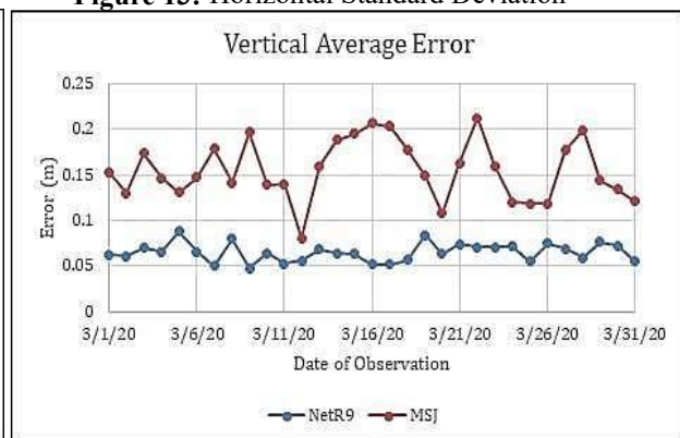
Figure 15: Vertical Average Error
