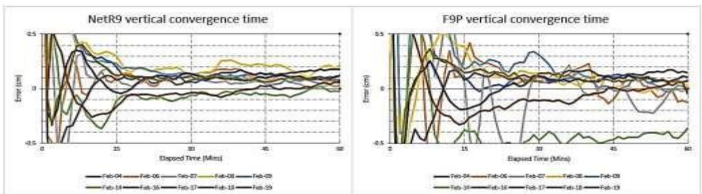
Figure 4: Trimble NetR9 and ZED-F9P vertical convergence time
