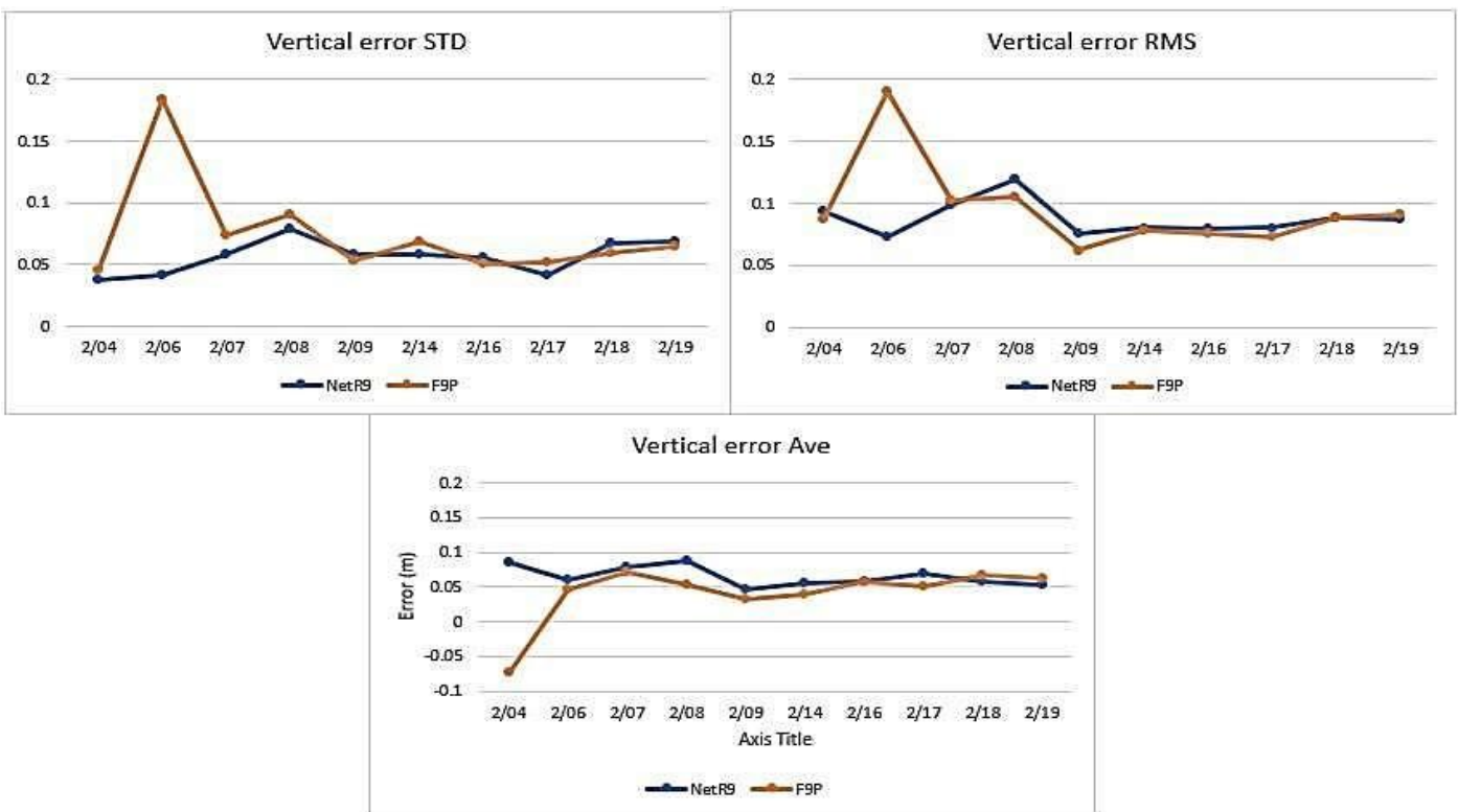
Figure 7: Vertical error statistics plot
