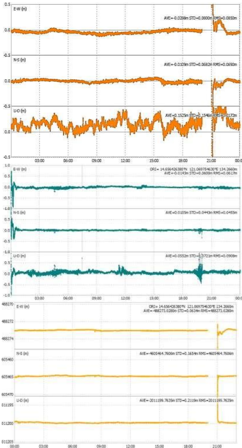
Figure 10: Real-Time solution of MSJ in Curtin University, Australia (March 1, 2020).
