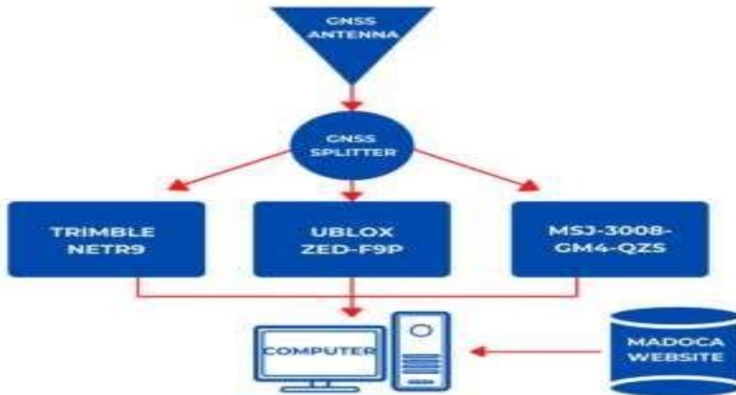
Figure 2: Data Gathering Setup
