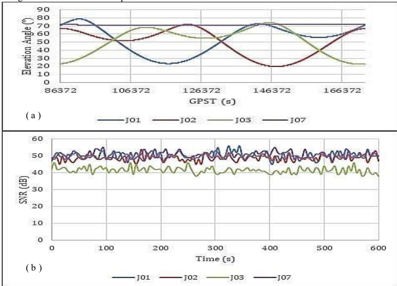
Figure 8: a) Elevation Angle of QZSS Satellites in UP Diliman (03/01/2020) and b) Signal to Noise Ratio of LEX signal during first 10 minutes
