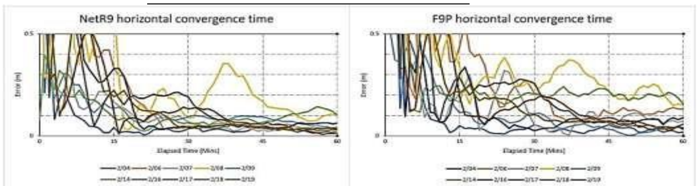
Figure 3: Trimble NetR9 and ZED-F9P horizontal convergence time
