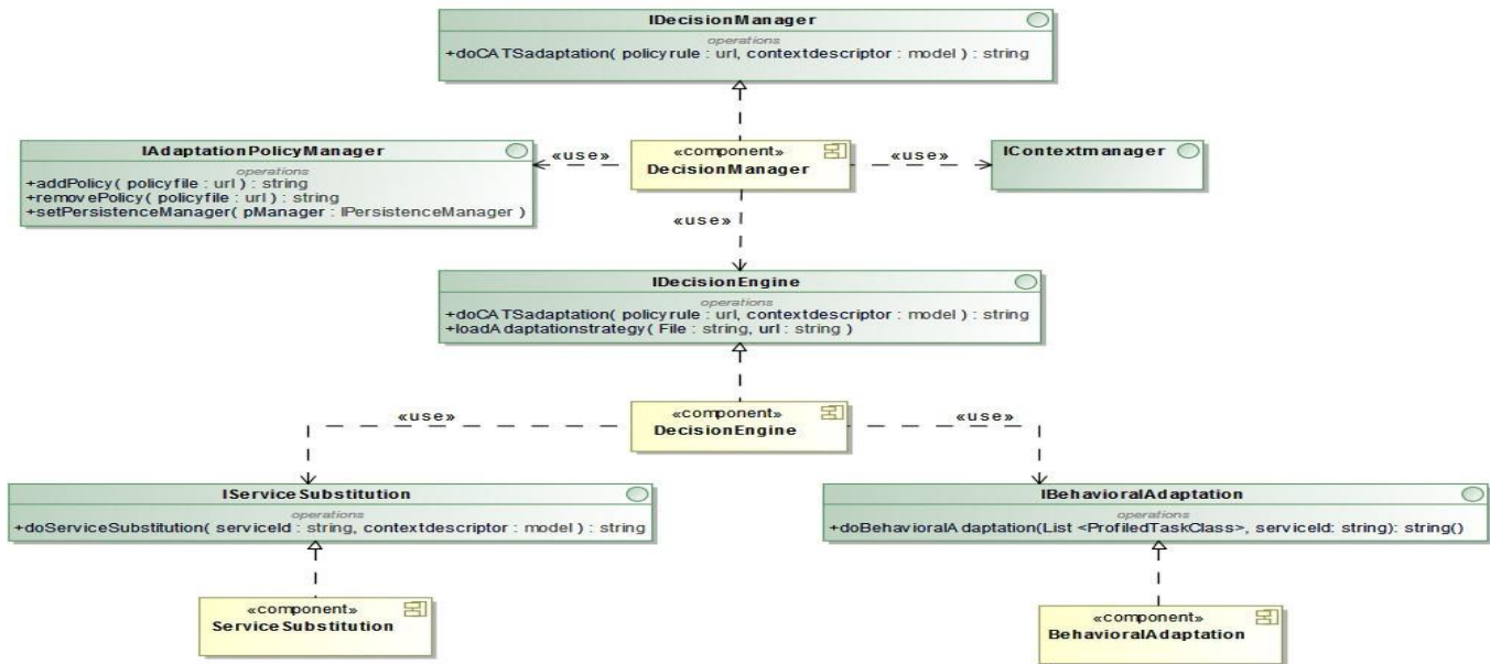
Fig. 4. Components implementing CATS service adaptation mechanism
