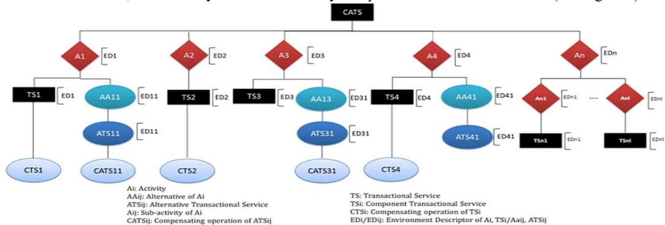
Fig. 1. Succinct illustration of CATS service structure
