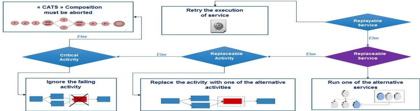
Fig. 6. CATS composition behavior according to activity profile
