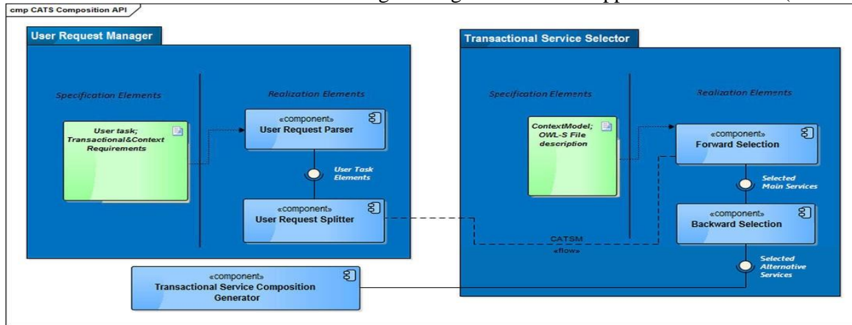
Fig. 3. CATS service composition API
