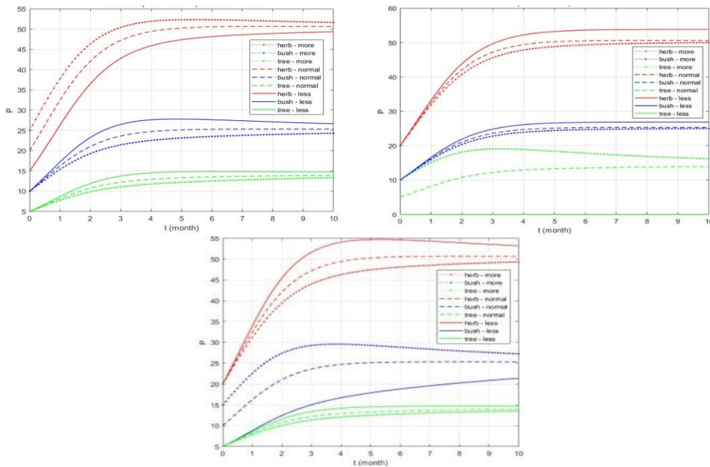
Figure 3: Relationships between Population and Different Plant Communities
