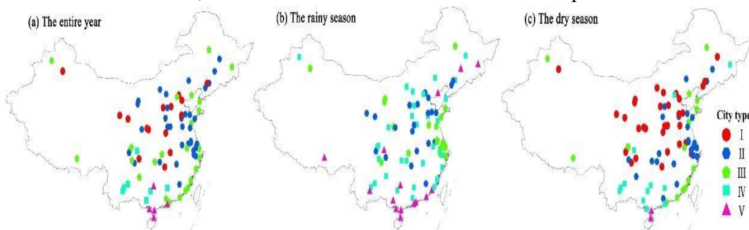
Figure 9: Temporal-spatial distribution characteristics of air-quality types at the different time scales.
