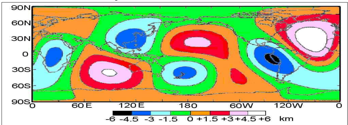
Figure 2. The topography of the CMB obtained by inversion of the combined PcP and PKP bc Data set.
