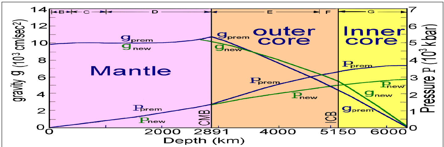
Figure 7. Diagram of the gravity g and the pressure P of the new Earth model and the PREM.
