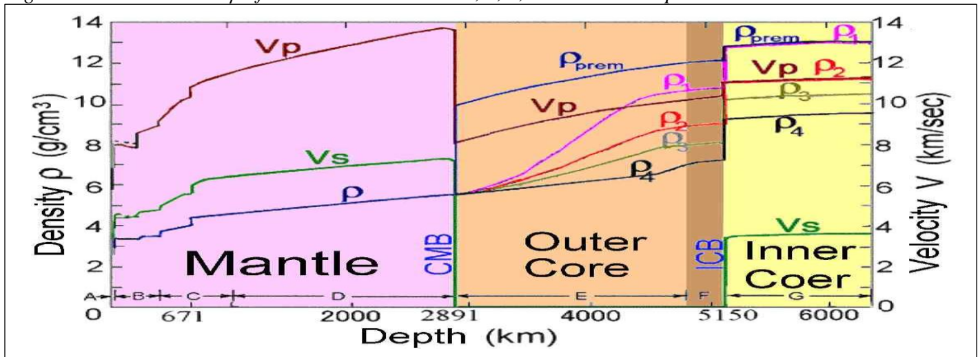
Figure 6. These densities \rho of the new Earth models 1, 2, 3, and 4 were compared with the PREM's.
