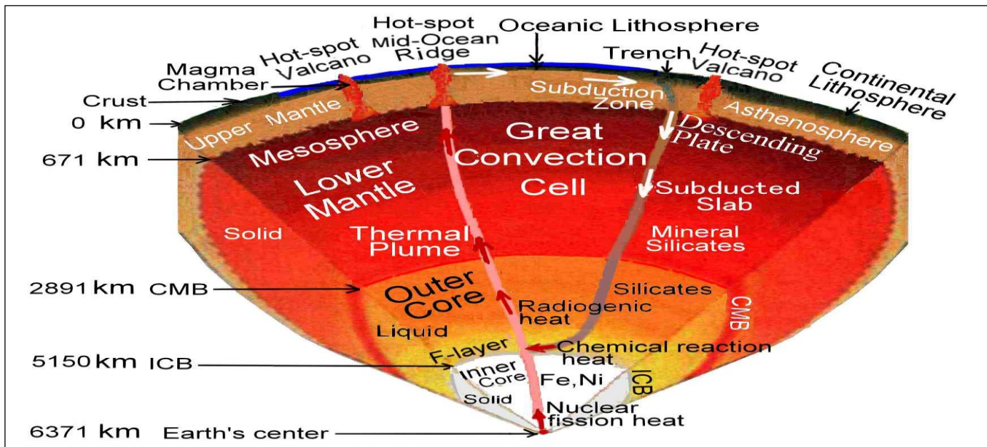
Figure 4. Schematic diagram of the great convection cell, heat flow, and the composition of Earth's interior.
