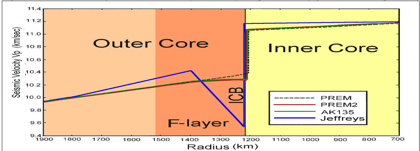
Figure 3. Variation chart of seismic wave velocity in the Flayer: V_p low-velocity gradient and sharp-velocity
