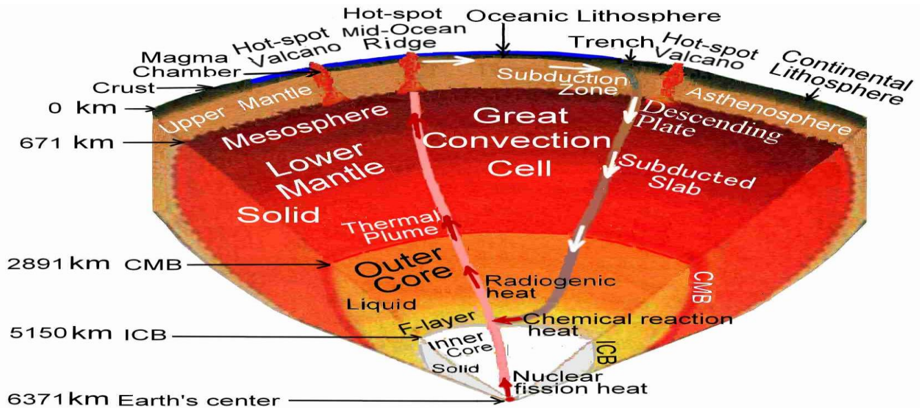
Figure 2: A schematic of the great convection cell, heat flow, and composition of the Earth's interior.
