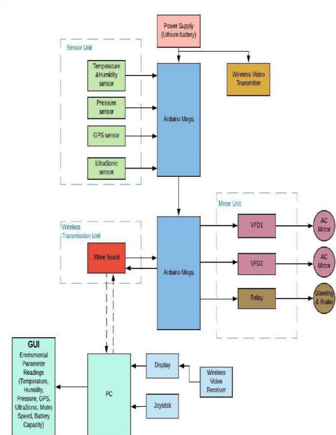
Figure 4 Sensors connected to Arduino Mega
