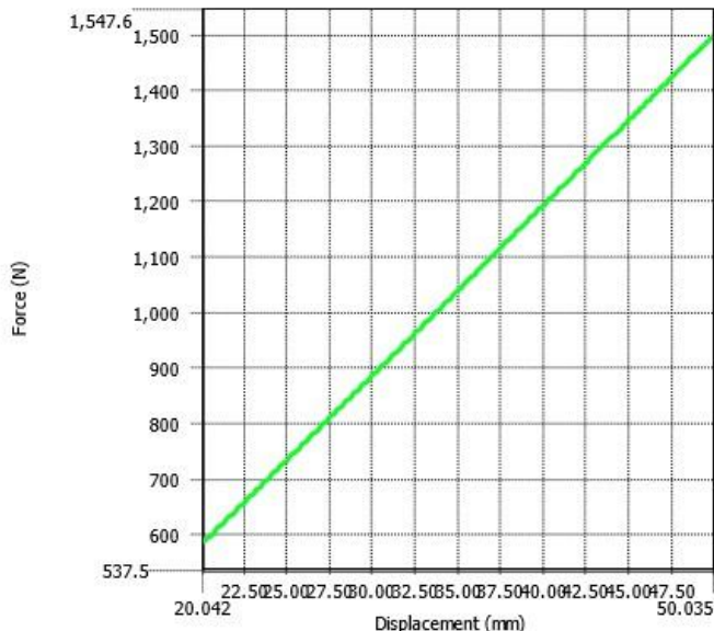
Figure 8. Rear wheels spring rate test 10mm preload and 25mm preload, respectively
