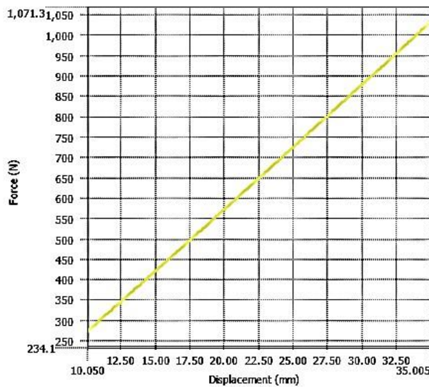
seeder-spring rate test-4 (30.57 N/mm)
