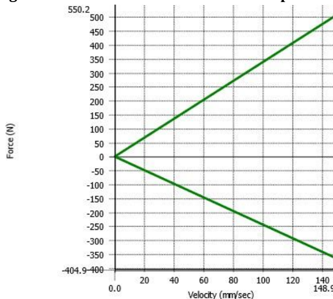
Figure 10. PVP absorber test, linear relationship in positive for compression and unfavorable for a rebound
