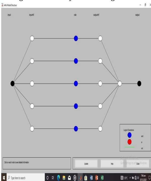
Fig 9.0: ANFIS Structure
