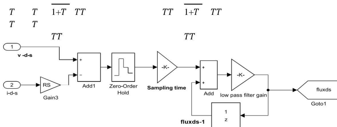
Figure 4: Digital Simulink block diagram for stator d axis flux in a stationary frame
