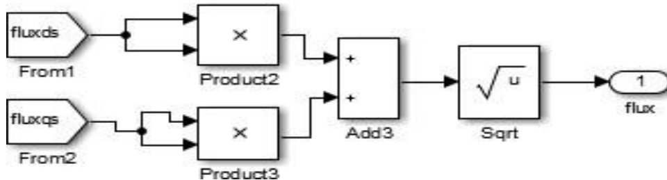
Figure 6: Resultant Stator flux calculation Simulink block
