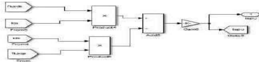
Figure 8: Torque estimator Simulink block
