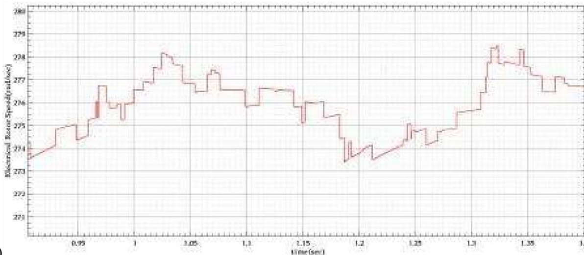
Figure 19: a) Estimated rotor speed without load torque b) rotor speed in zoom view
